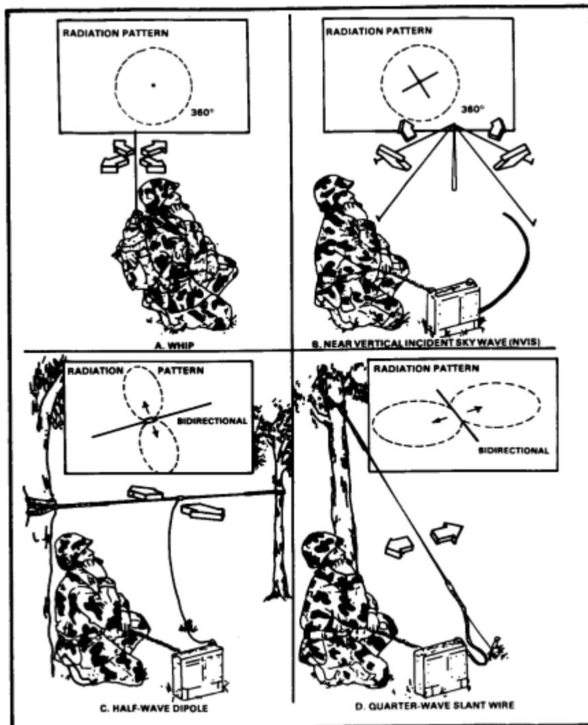
Figure 3-2. Antenna radiation patterns.
