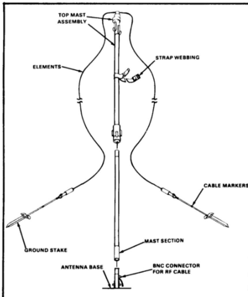
Figure 3-18. AS-2259/GR antenna base.
