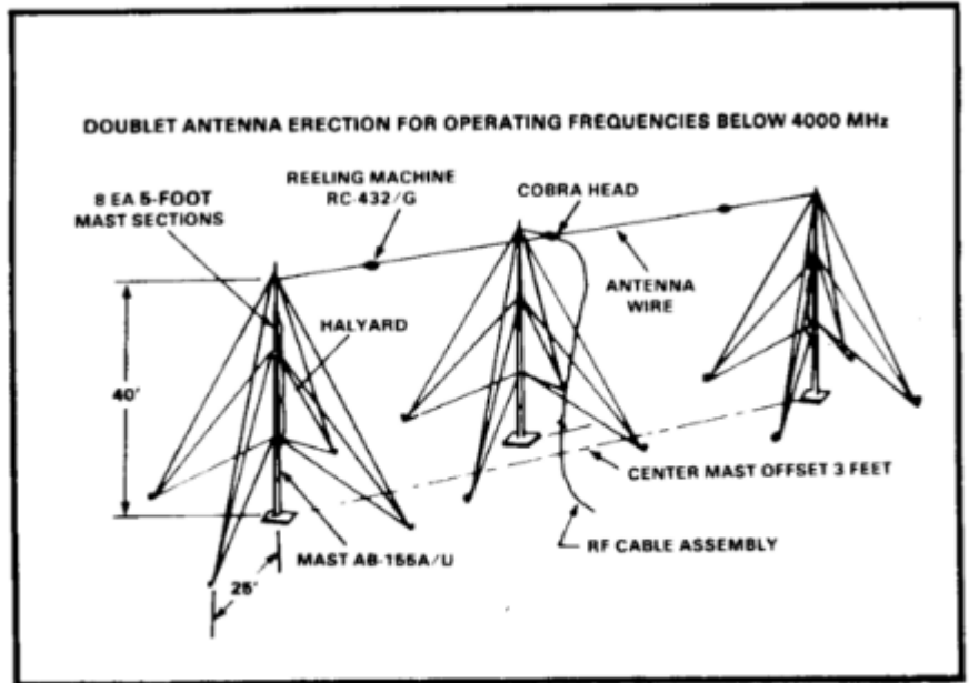
Figure 3-15. Doublet antenna installation using AB-155A/U. (continued)
