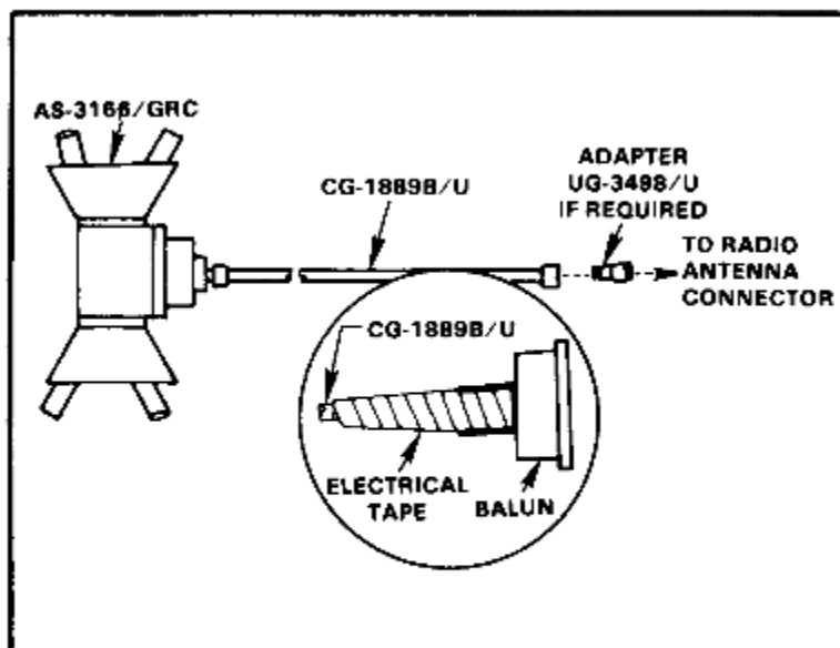
Figure 3-12. Connections of CG-1889B/U to AS-3166/GRC and radio.
