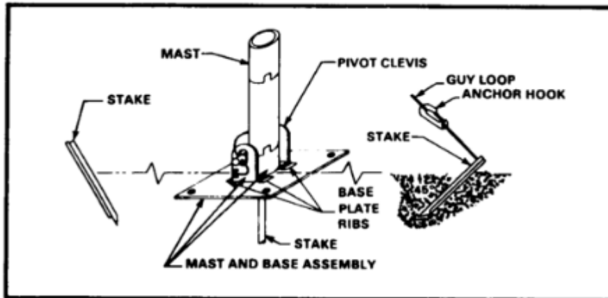
Figure 3-4. Ground anchor/pivot clevis alignment.
