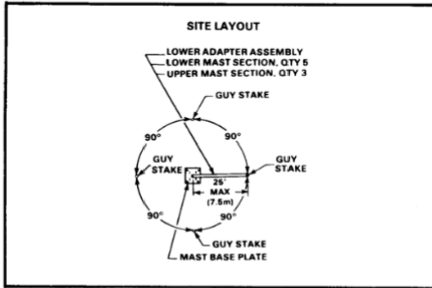
Figure 3-3. Positioning guy stakes.
