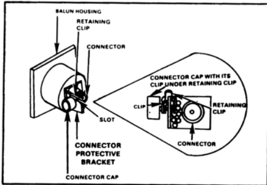
Figure 3-11. Captivating feed cone assembly connector cap.
