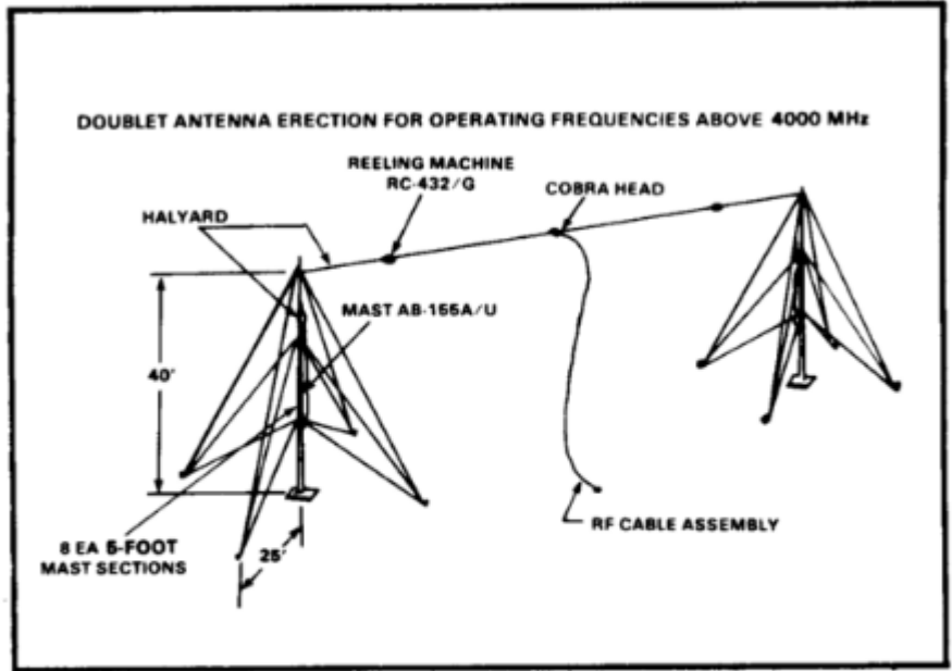
Figure 3-15. Doublet antenna installation using AB-155A/U.
