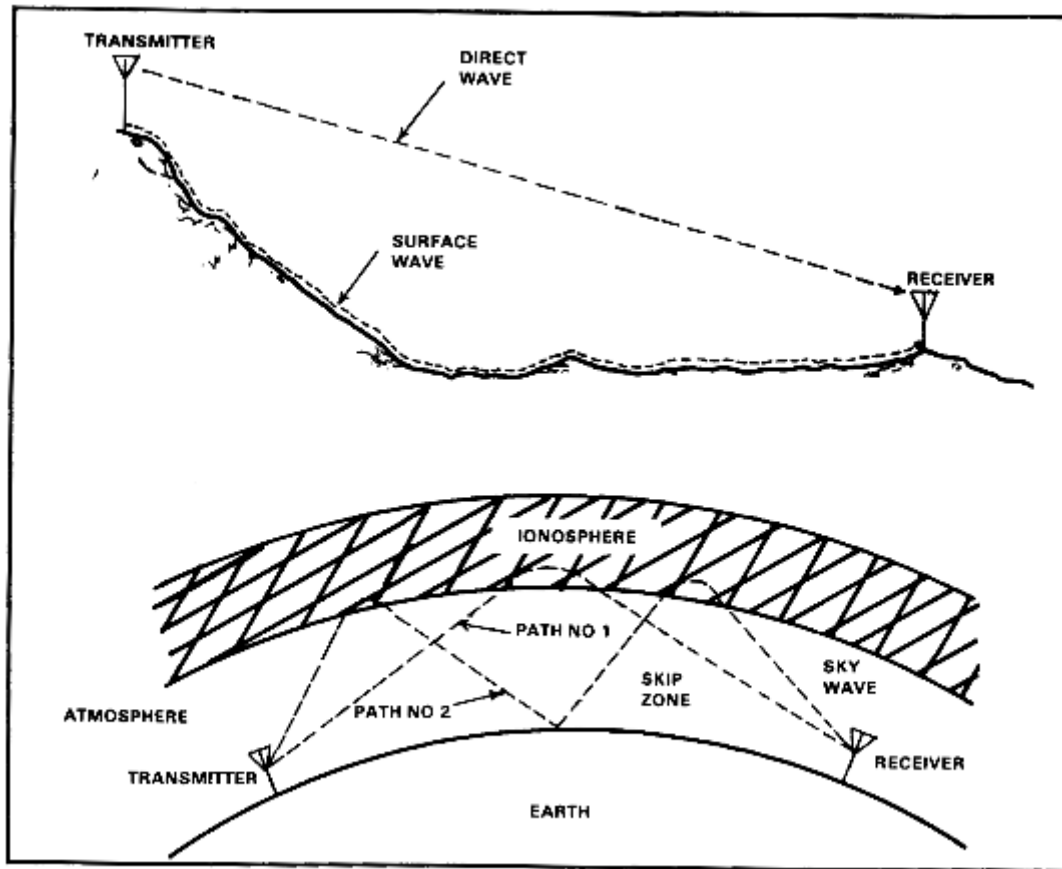
Figure 3-1. Sky-wave and ground-wave propagation.
