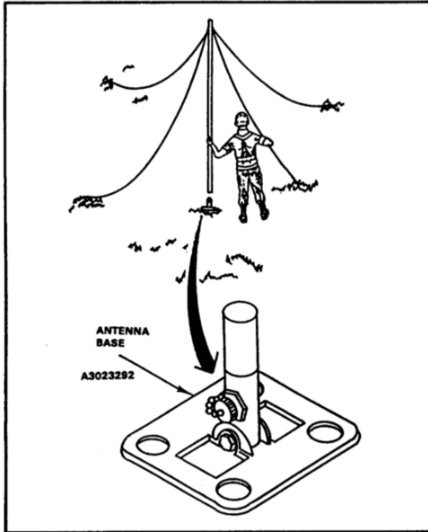
Figure 3-19. AS-2259/GR antenna top mast assembly installation.
